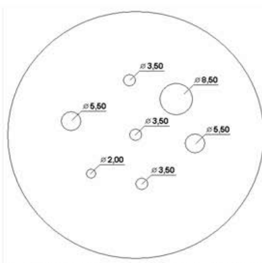
Standard probe hole dimensions at depth 77mm
